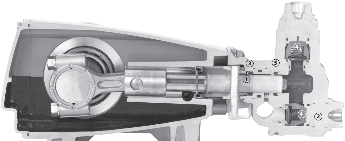
Models 70, 70G1
