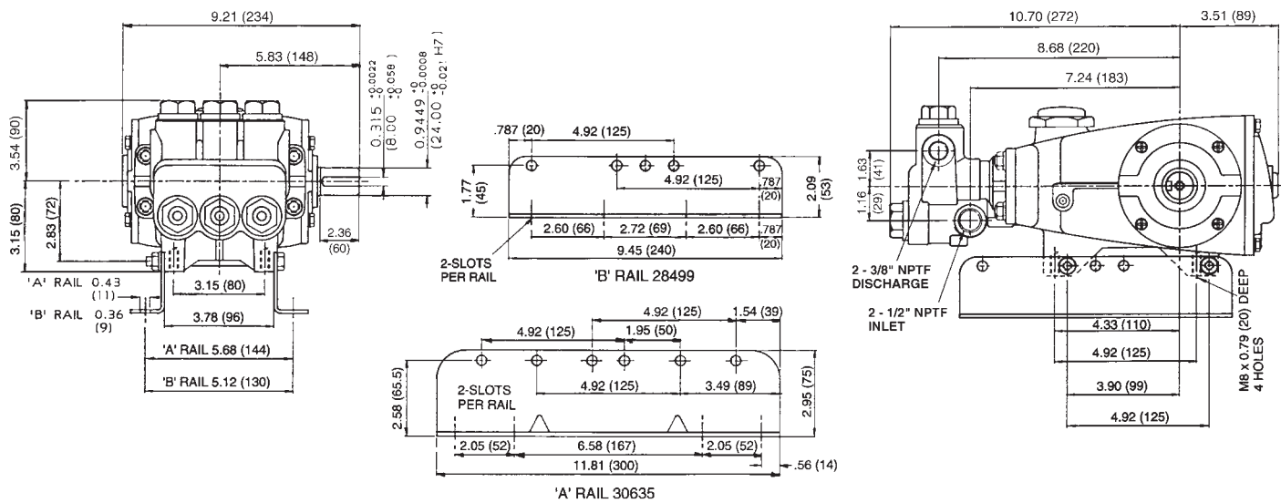
Models 70, 70G1
